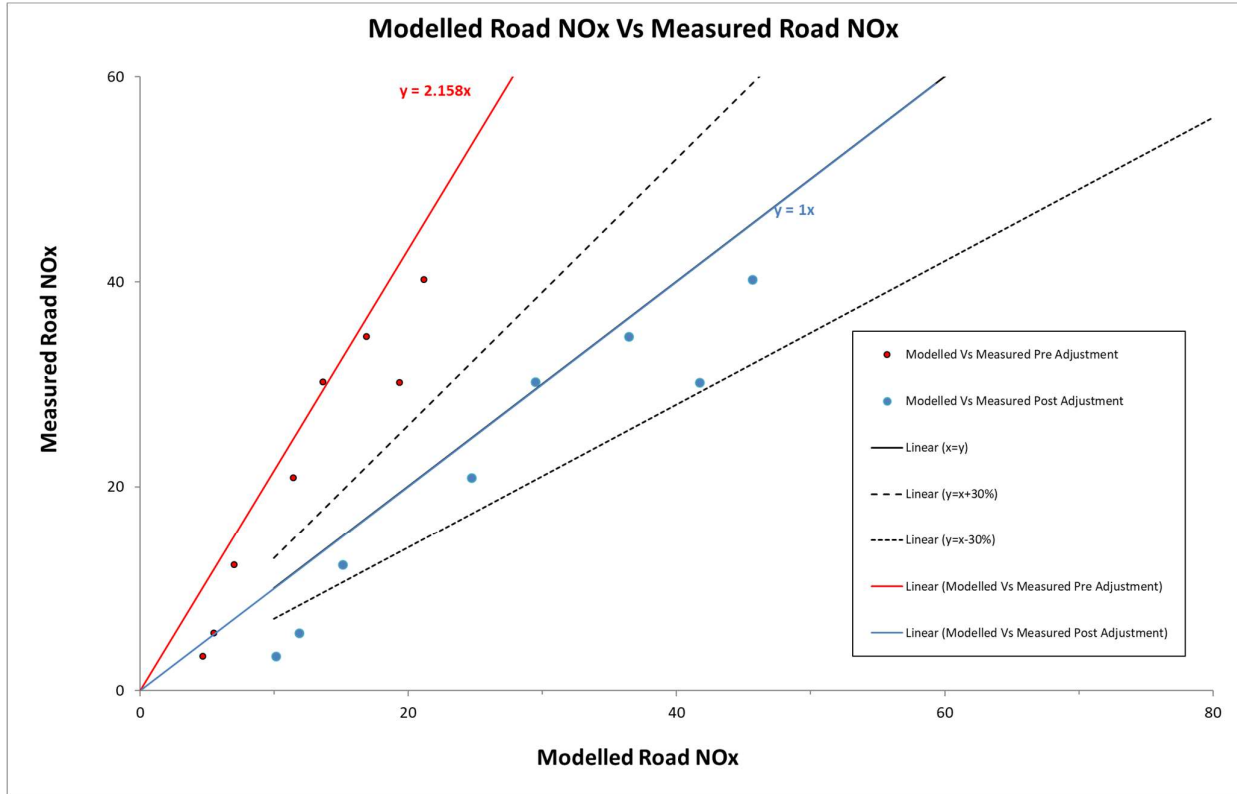
Figure 1: Linear regression plot of modelled vs monitored NO x 2015 –scheme specific monitoring
